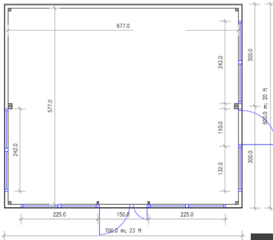
Floor plan
