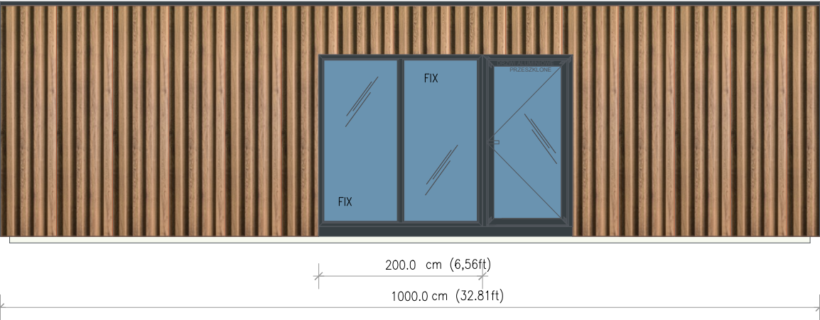
REAR WALL
